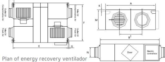
Plan of energy recovery ventilator
